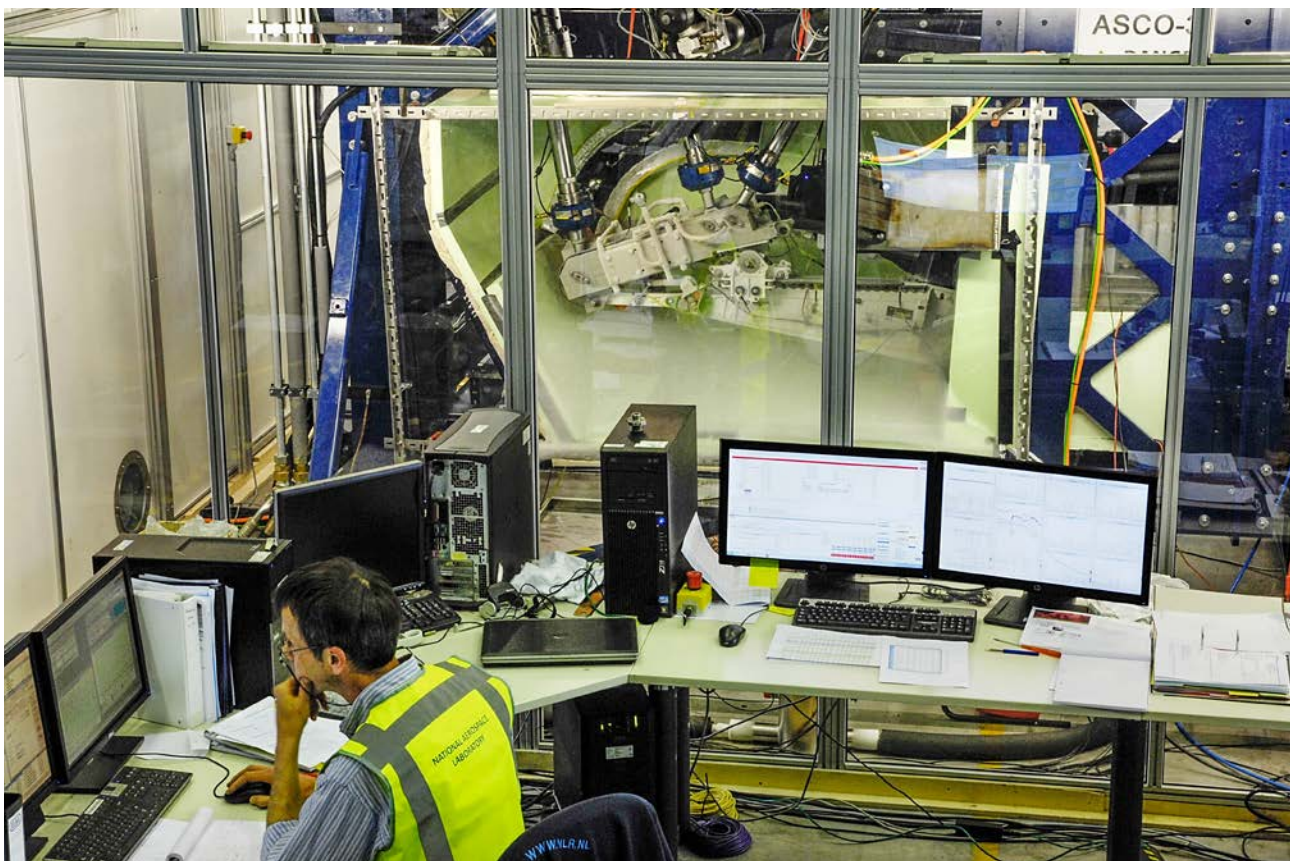
Overview of full scale flap track test setup at -55°C.
